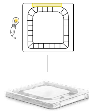
COPERCHIO/LID x L.2,3 Art. 2300-CB ● 18x16,5 - PET/THF 336pcs(2x168pcs)
